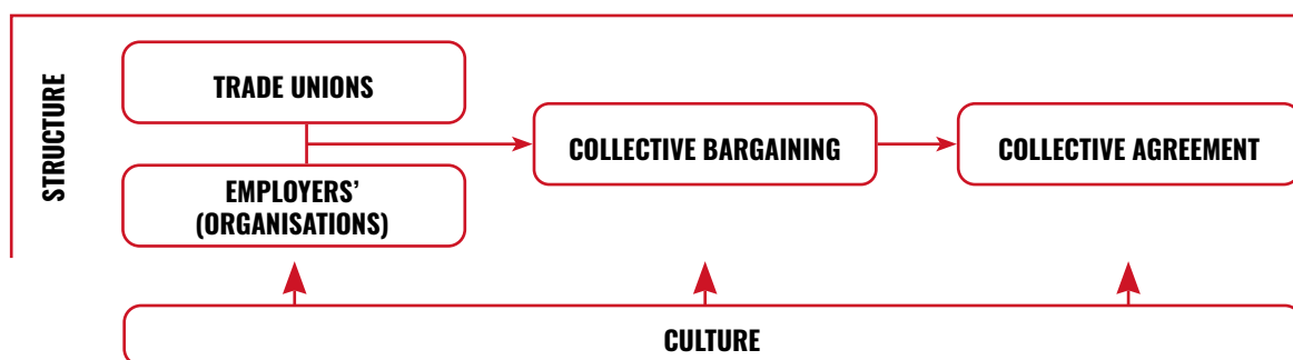
Figure 3 - Analytical framework
